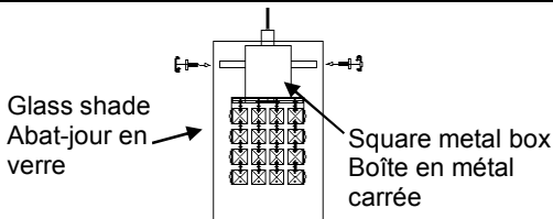
Bulb Ampoule
